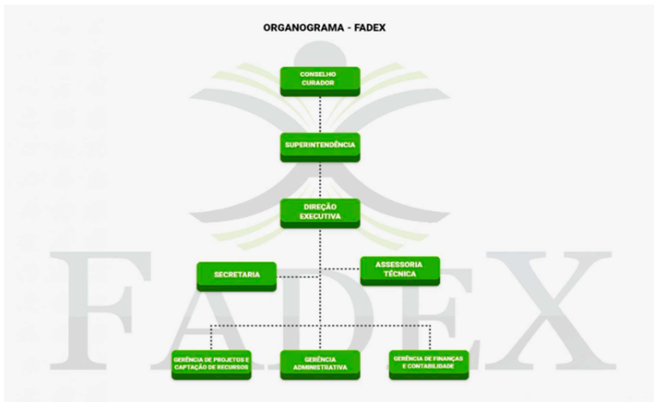
Figura 1 - Organograma Fadex
